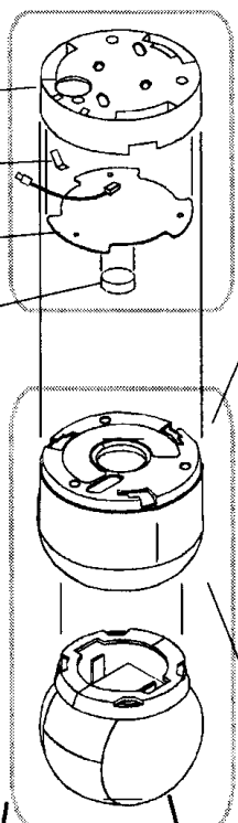
Figure Chapter 1-2. Dome components
